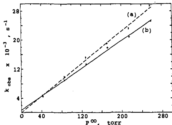
Figure 5. Determination of k^{\text{CO}} for the equilibrium: \text{Fe}(\text{durene-5/5})\text{-(DcIm)} + \text{CO} \rightleftharpoons \text{Fe}(\text{durene-5/5})(\text{DcIm})(\text{CO}) at 20 °C in toluene. Data measured at (a) 425 nm, gives k^{\text{CO}} = 111.8 \text{ Torr}^{-1} \text{ s}^{-1} and at (b) 415 nm, gives k^{\text{CO}} = 95.7 \text{ Torr}^{-1} \text{ s}^{-1} . Average k_{\text{DcIm}}^{\text{CO}} = 1.1 \times 10^7 \text{ M}^{-1} \text{ s}^{-1} .
