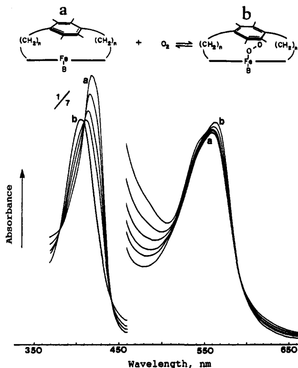
Figure 3. Isosbestic spectral changes in the 360–650-nm region for the equilibrium: Fe(durene-4/4)(N-MeIm) + O 2 ⇌ Fe(durene-4/4)(N-MeIm)(O 2 ) at 20 °C in toluene; added P_{\text{O}_2} = 24, 64, 124 Torr and final pressure of 1 atm.
