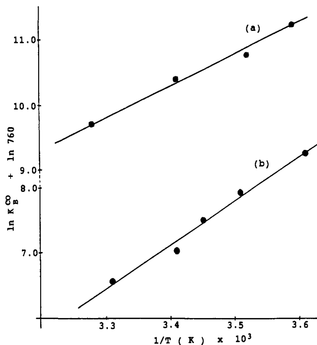
Figure 2. van't Hoff plots for the equilibria: Fe(durene-4/4)(B) + CO = Fe(durene-4/4)(B)(CO) measured in toluene from 0 to 30 °C. (a) B = DcIm, gives \Delta H^{\circ} = -9.4 kcal/mol and \Delta S^{\circ} = -11.6 eu. (b) B = 1,2-Me 2 Im, gives \Delta H^{\circ} = -13.7 kcal/mol and \Delta S^{\circ} = -32.4 eu.
